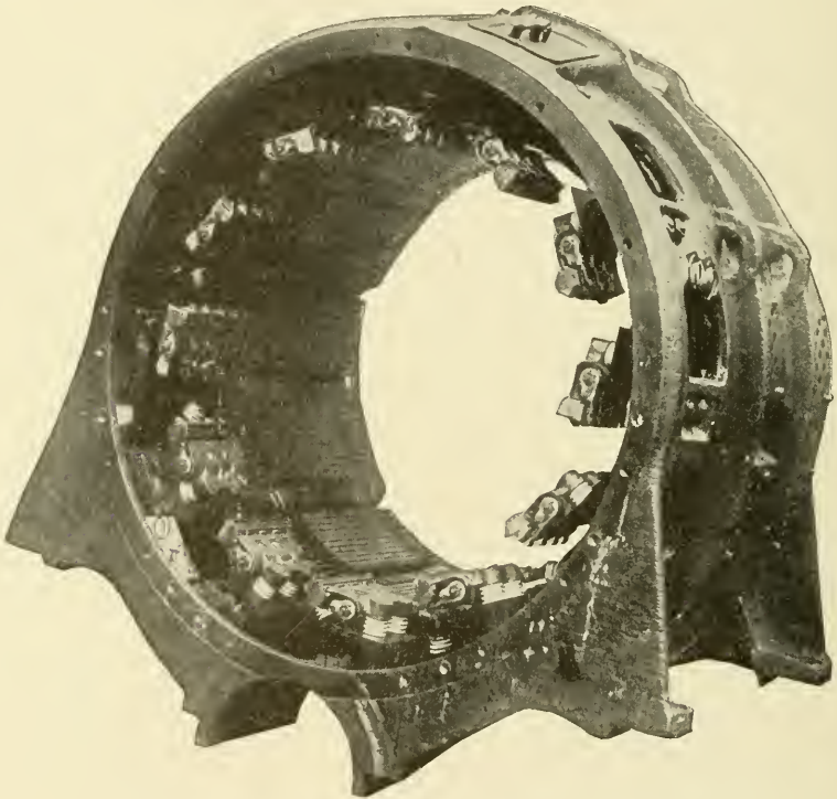
Fig. 262. Field Circuits and Brush Holders of Motors Shown in Fig. 261
